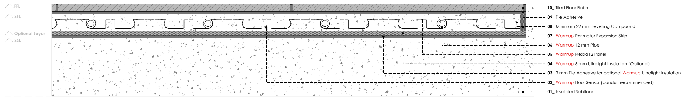
WARMUP NEXXA12 SYSTEM. Tiled floor finish
