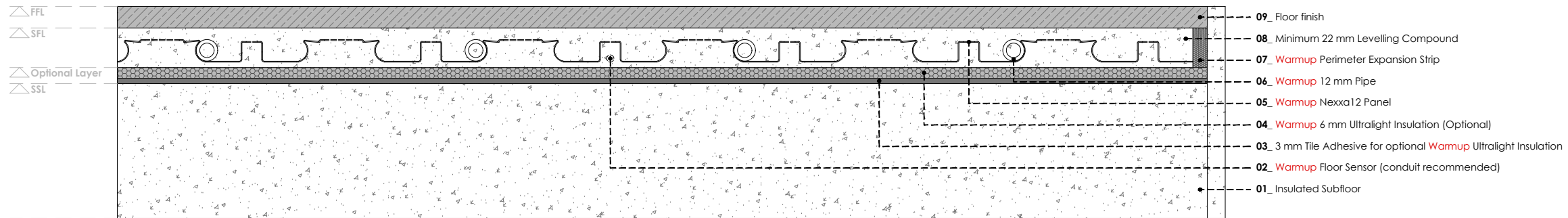
WARMUP NEXXA12 SYSTEM. Standard Detail
