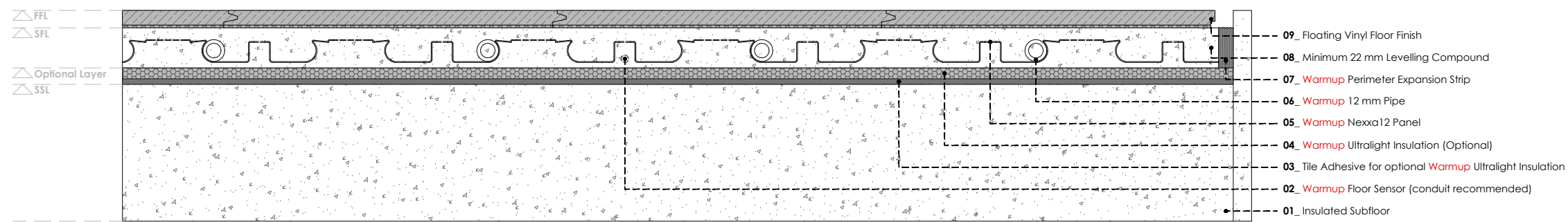
WARMUP NEXXA12 SYSTEM. Vinyl floor finish - floating
