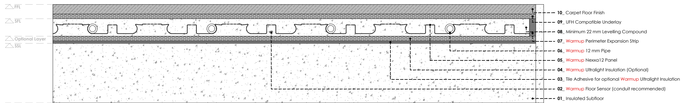
WARMUP NEXXA12 SYSTEM. Carpet floor finish
