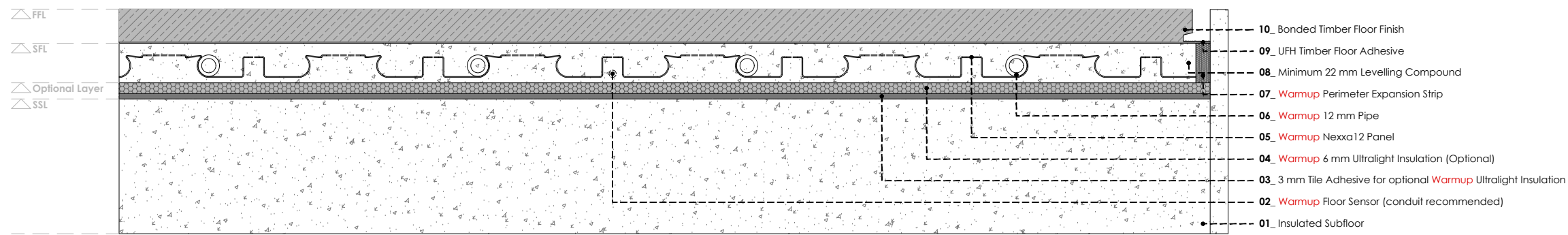
WARMUP NEXXA12 SYSTEM. Bonded timber floor finish
