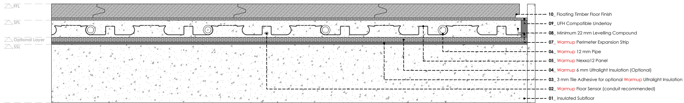
WARMUP NEXXA12 SYSTEM. Floating timber floor finish
